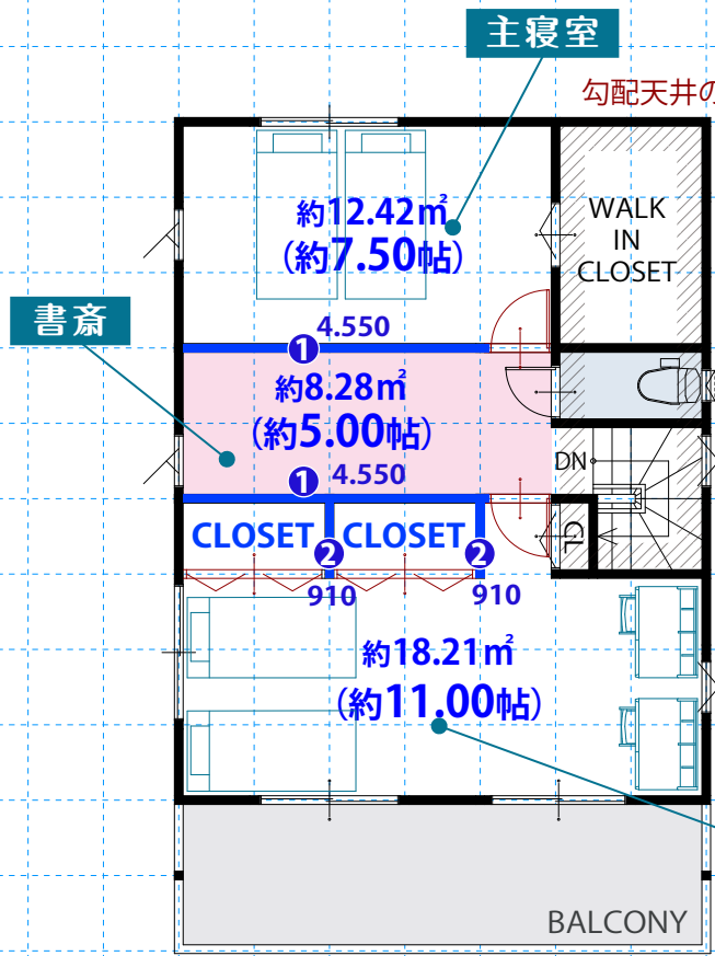
2 FLOOR / 52.17㎡
