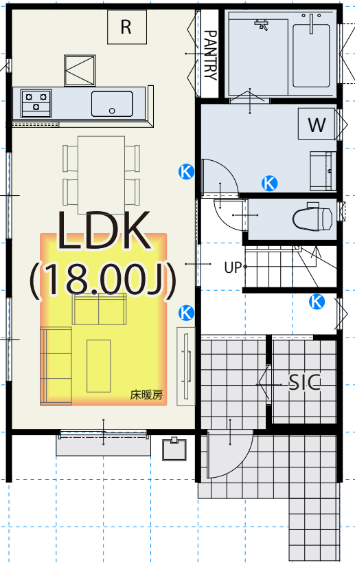
1 FLOOR / 52.17㎡
