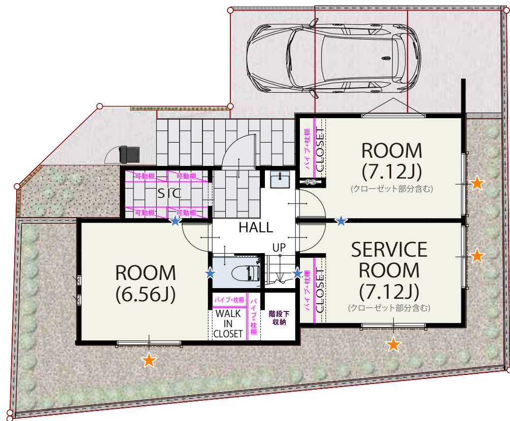
1 FLOOR / 47.92㎡
