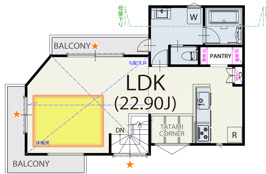
2 FLOOR / 52.63㎡
