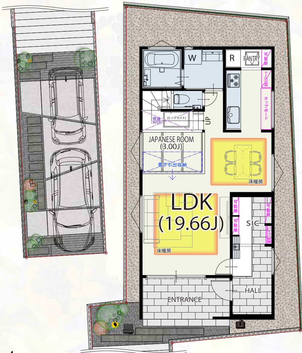
1 FLOOR / 62.37㎡
