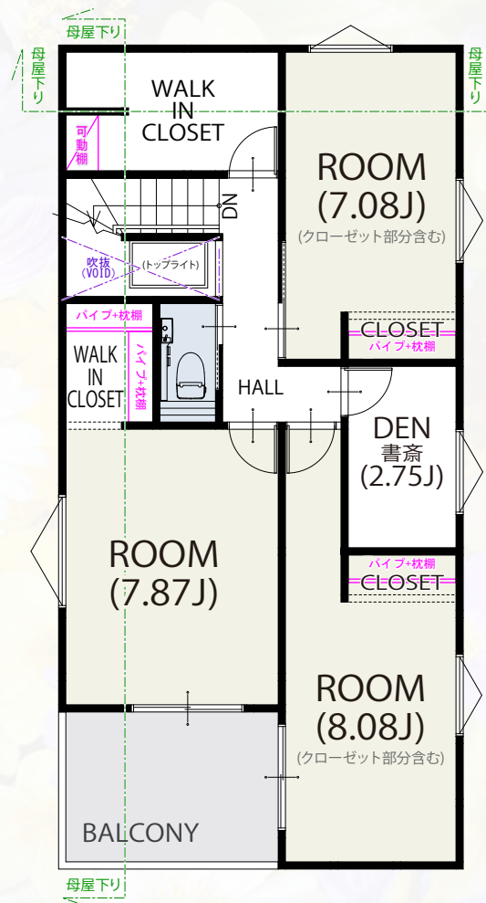
2 FLOOR / 60.93㎡
