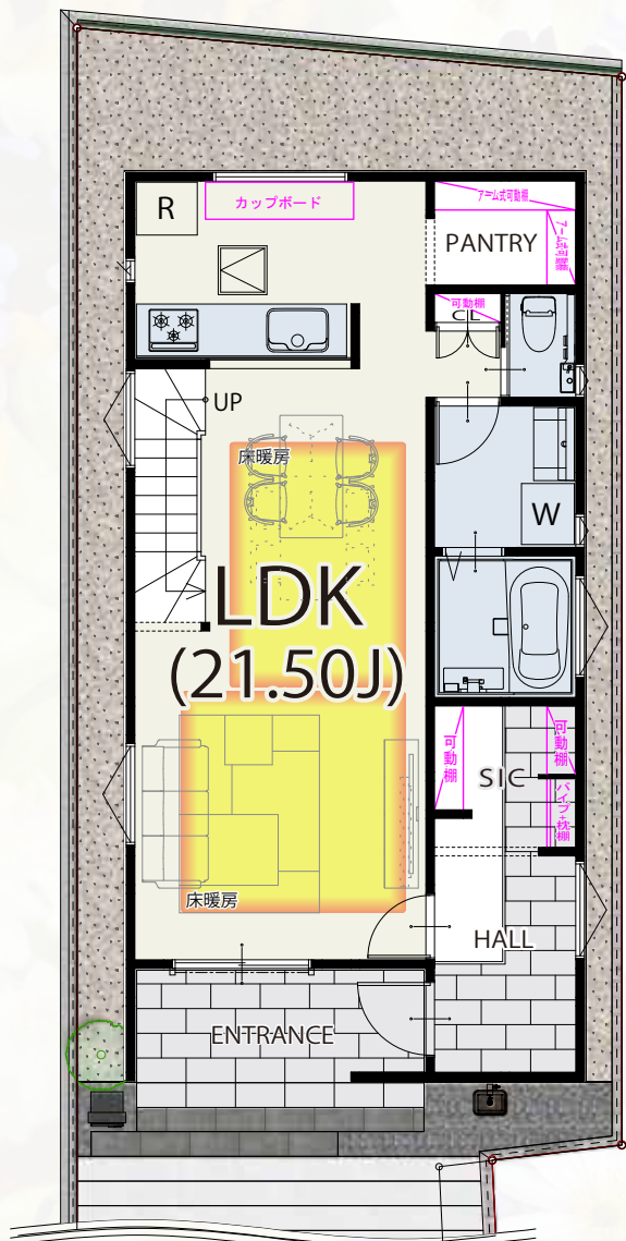
1 FLOOR / 55.89㎡
