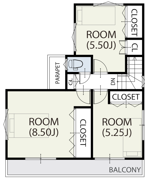
2 FLOOR / 43.88㎡
