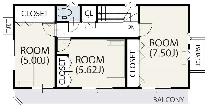
2 FLOOR / 43.47㎡
