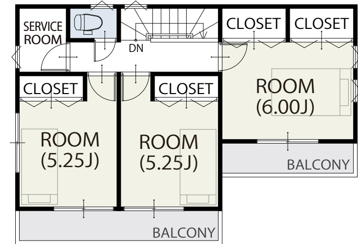
2 FLOOR / 43.06㎡
