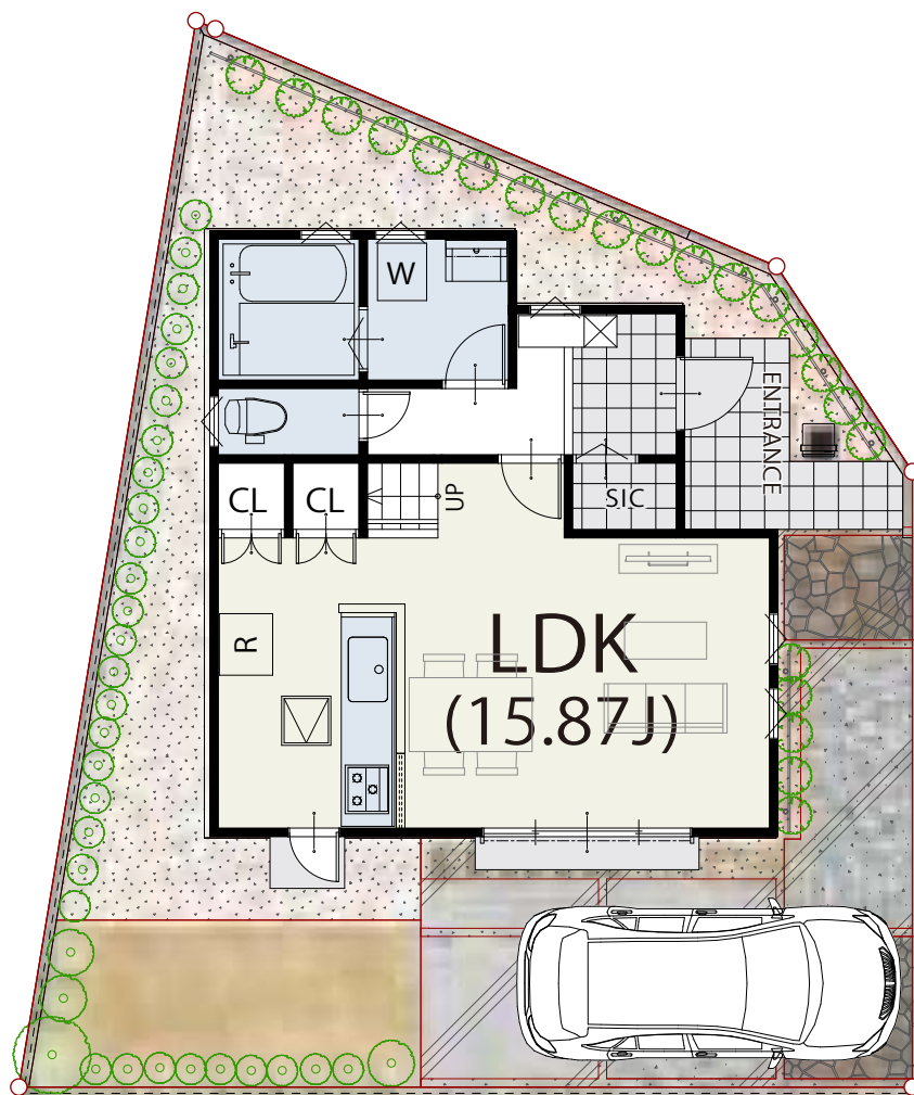
1 FLOOR / 43.68㎡
