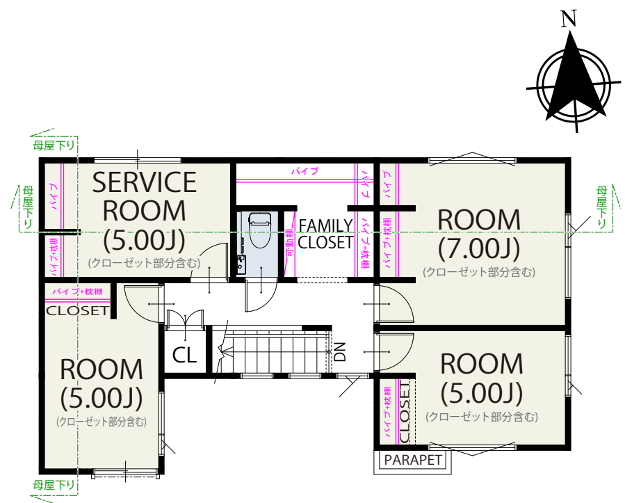
2 FLOOR / 50.10m 2
