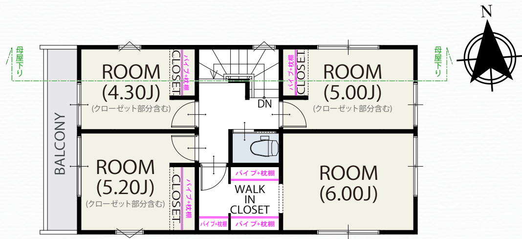
2 FLOOR / 45.54m²
