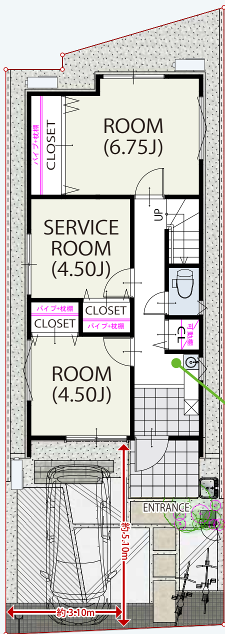
1 FLOOR / 42.64㎡
