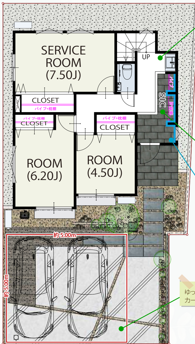
1 FLOOR / 49.61㎡
