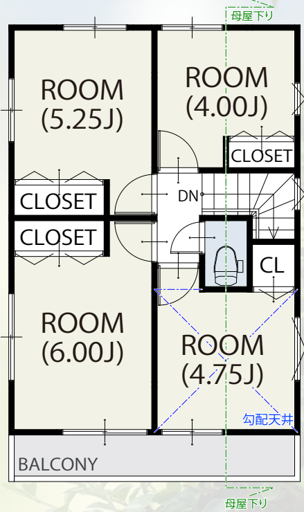
2 FLOOR / 42.23㎡
