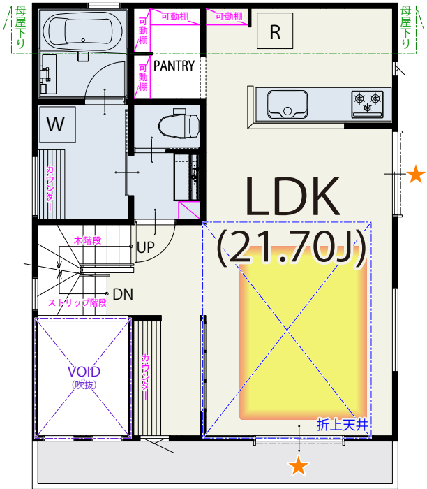
2 FLOOR / 51.75m 2
