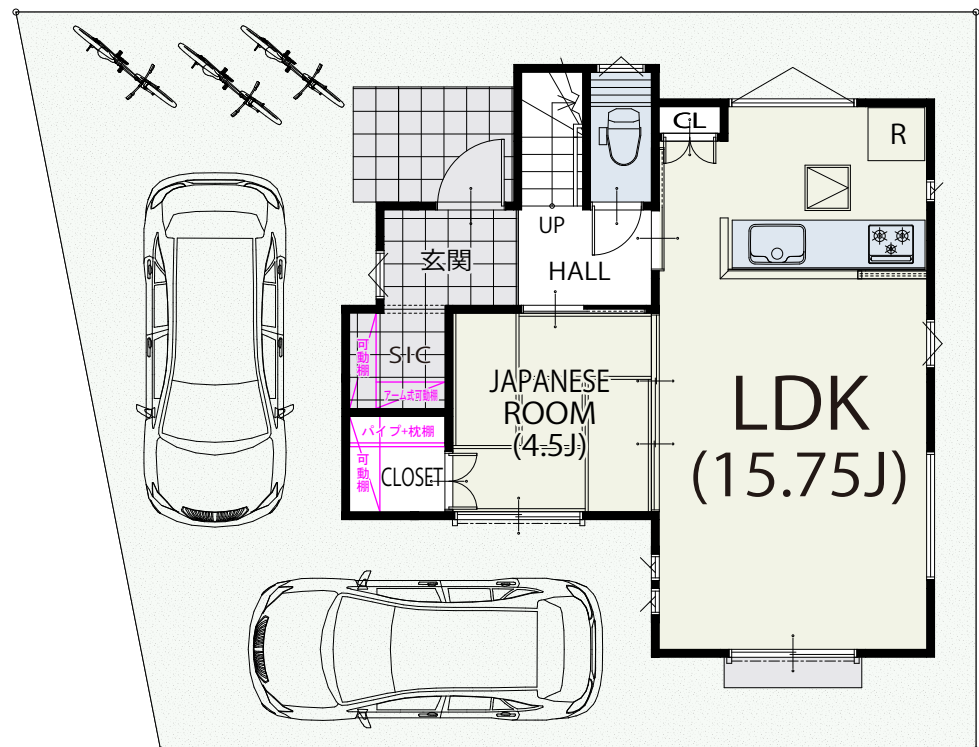
1 FLOOR / 45.95㎡
