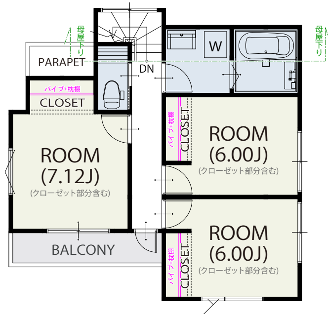
2 FLOOR / 46.16㎡
