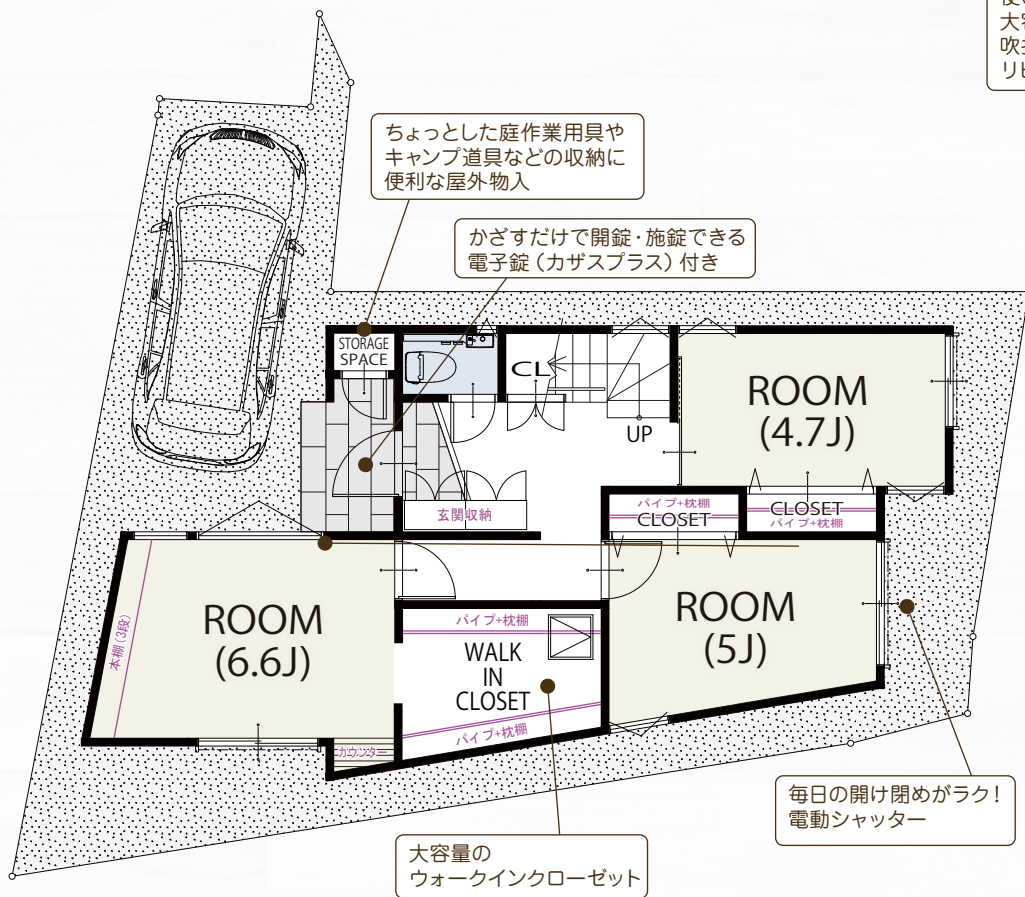
1 FLOOR / 46.76m 2
