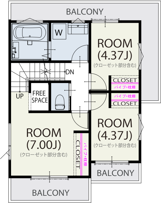
2 FLOOR / 40.16m²
