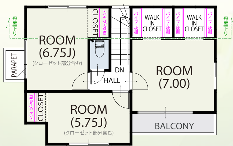
2 FLOOR / 42.64㎡
