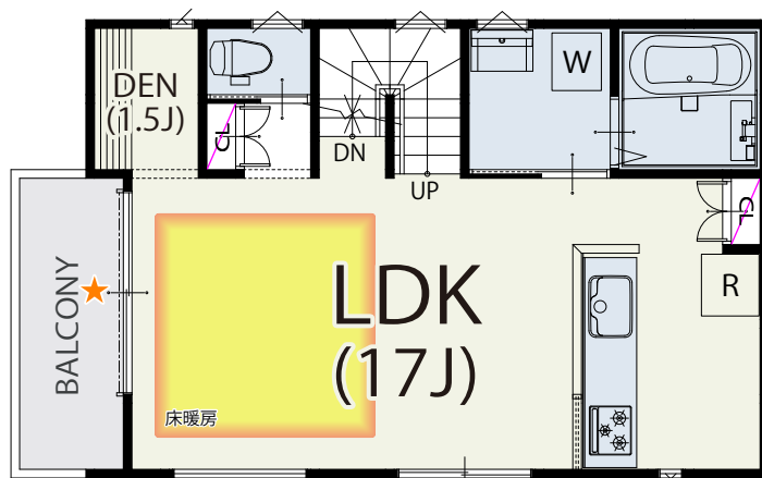
2 FLOOR / 43.06㎡
