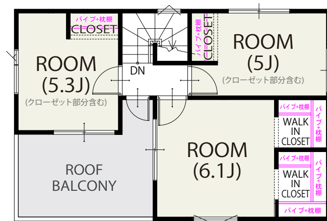
3 FLOOR / 36.43㎡
