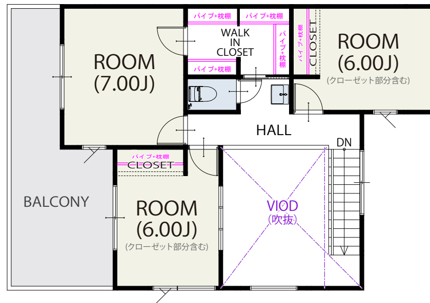
2 FLOOR / 45.59m 2
